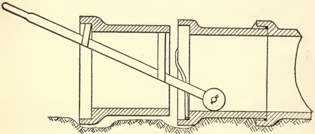
FIG. 20.—APPLIANCE FOR "ENTERING" HEAVY PIPE.
